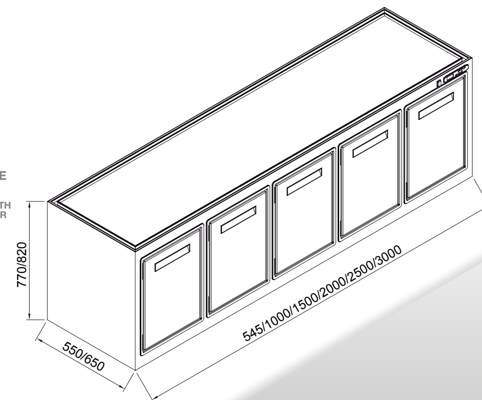
CELLA STATICA TN STATIC REFRIGERATOR UNIT
